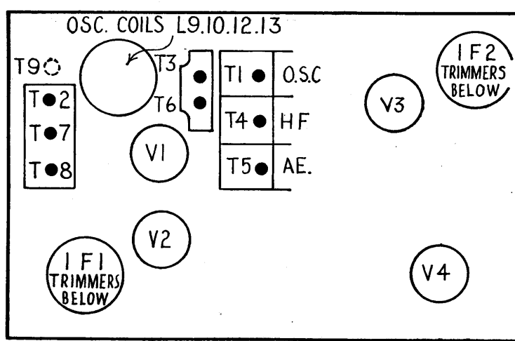
Top-of-chassis layout diagram of the Ekco BAW71, showing how the trimmers, valves, and some of the coils are located. The image rejector, T9, is adjustable from the front of the set.
