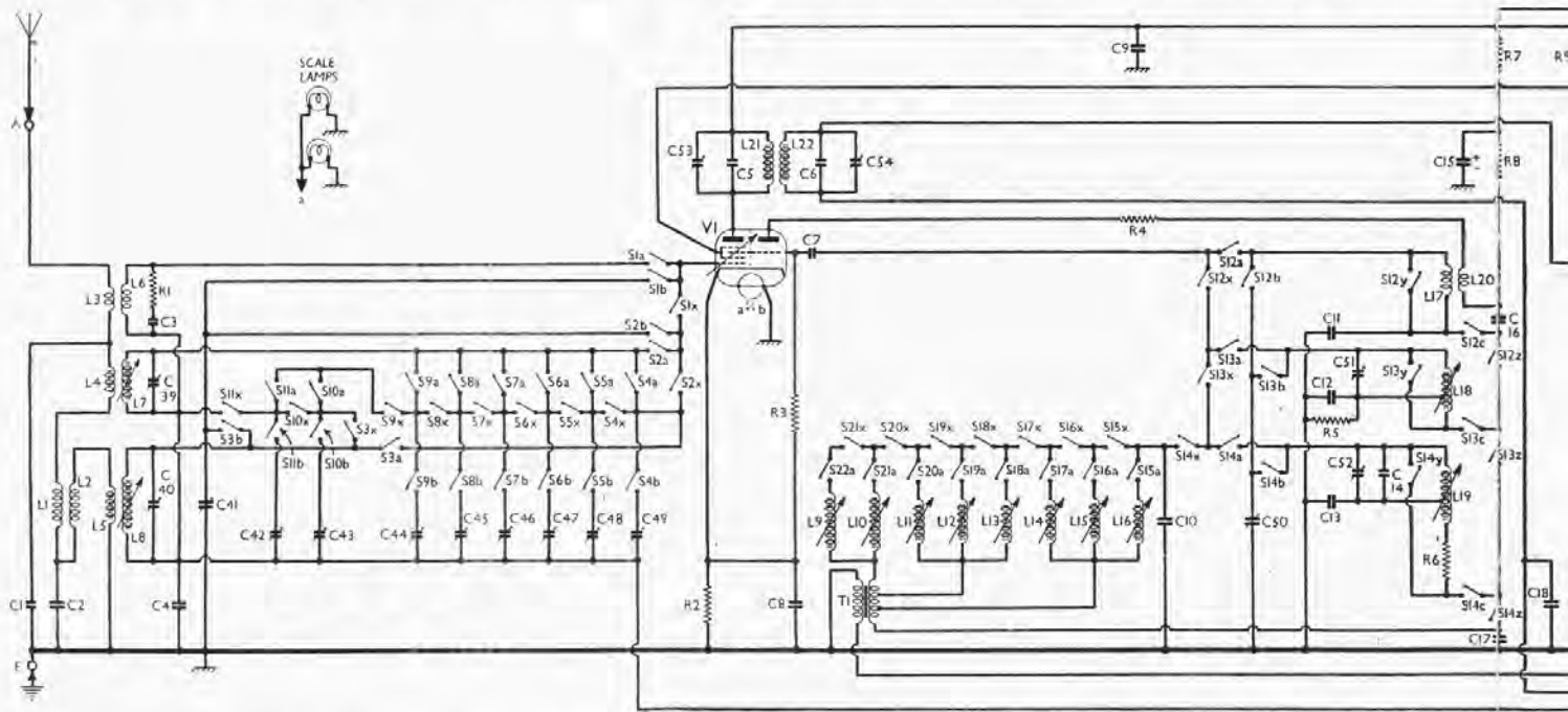
Circuit diagram of the Marconiphone 874 and H.M.V. 1102. In the press-button section, condenser trimmers are used for the aerial coils for the oscillator circuit. V8 is the double-diode AFC discriminator valve, which has two separate cathodes. T1 is the AFC control transformer; its pick-up socket is split.
