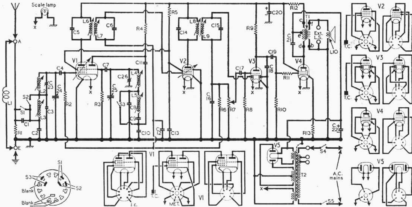
Circuit diagram of the G.E.C. BC5243 A.C. superhet, with the waveband switch inset below. Inset also are diagrams of the alternative valves, with three different types for V1. T1 connections are coded to agree with the markings in our plan view overleaf.
