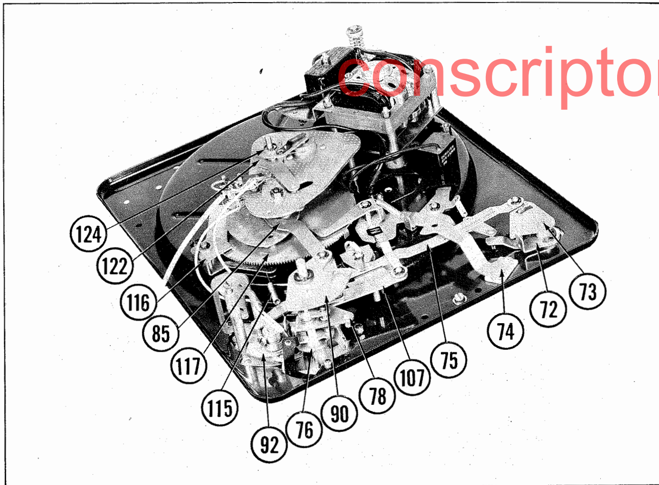
FIG. 3 TILTED BOTTOM VIEW OF CHANGER MECHANISM
