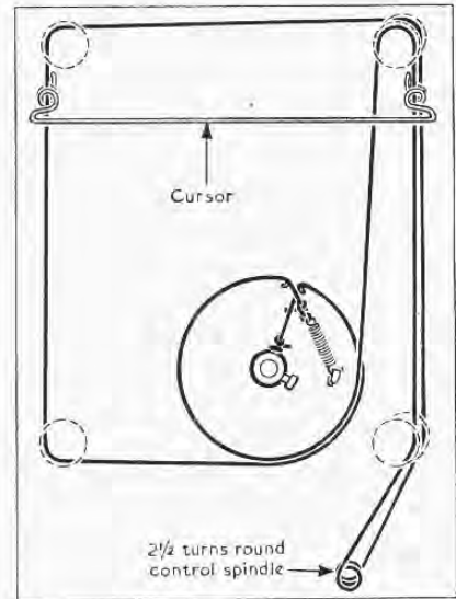
Above: Sketch of the tuning drive system. Below: Under-side illustration of the chassis.
