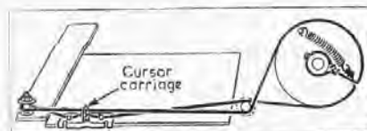
Sketch showing the tuning scale cursor drive cord, drawn as seen when viewed from the tuning knob end of an inverted chassis after removing the knob. The gang is at maximum.
