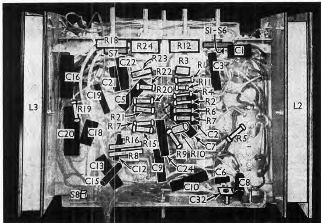
Under-chassis view. The S1-S6 switch unit is indicated here but in the diagram opposite it is drawn as seen in the plan view overleaf. Most of the resistors are mounted in two assemblies near the centre, and C2, C5 and C7 are beneath them in this view.
