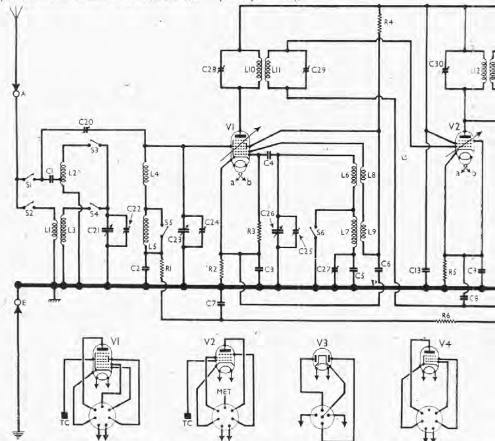
Circuit diagram of the Ekco AC77 AC superhet and the console model CT77. The separate parts are connected to the chassis by connections numbered 1 to 10. These numbers are repeated in our illustration of the unit of the section of the mains transformer.
