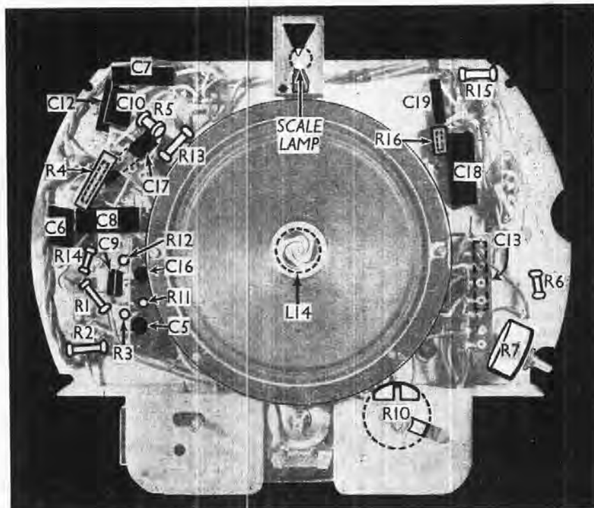
Front view of the chassis. Most of the small components are seen here distributed round the speaker, which is mounted on the chassis. C13 is hidden by the terminal strip on the right.
