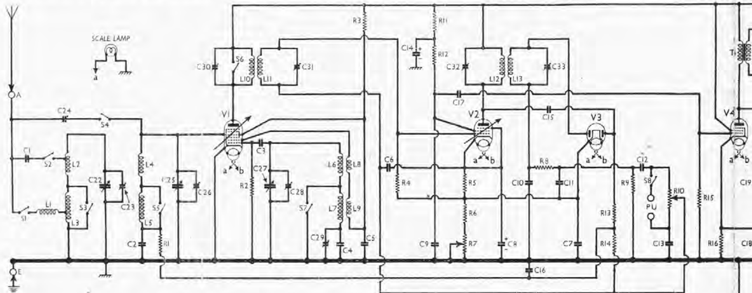
Circuit diagram of the Ekco AC76 superhet. V2 , in addition to acting as an IF amplifier in the normal manner, amplifies as an audio frequency amplifier, signals from the diode circuit being fed back to it via R10 , when the SG functions as a triode anode. It also forms the major part of a noise suppressor circuit, signal diode bias being obtained from R6, R7 . S6 closes on gram to mute radio signals.
