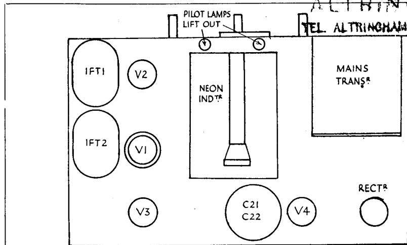
There are no trimmers on the gang condenser of the S.A.C.5. They are fitted to the coils and are adjusted from below the chassis.
